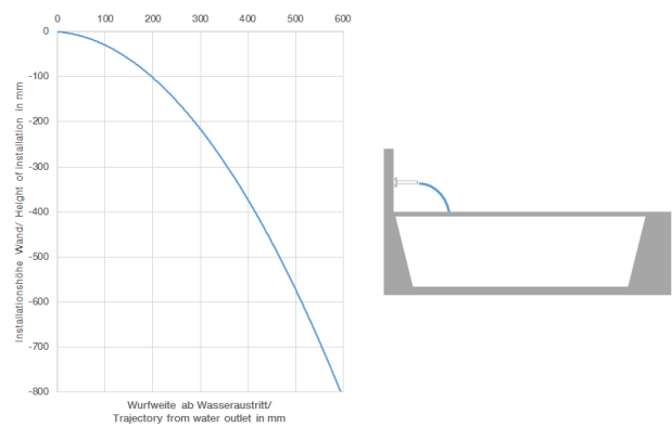
Trajectory diagram
